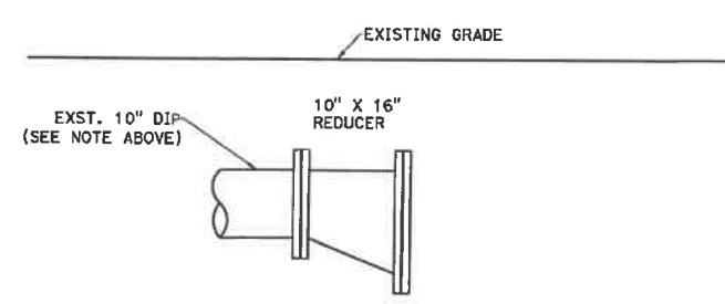
A REDUCER SECTION Scale: 1" = 2'
