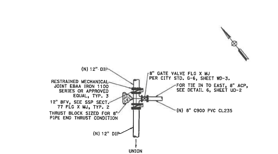
3 WATERLINE TIE-IN DETAIL - 2900 UNION ROAD Scale: 1" = 5'
