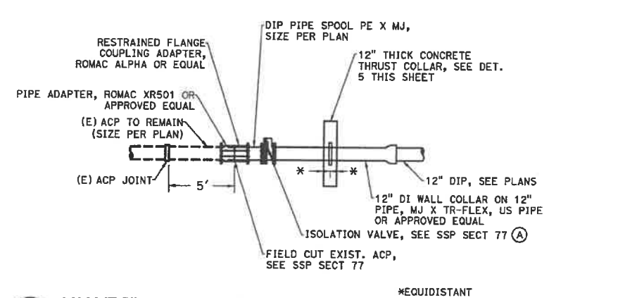
4 VALVE TIE-IN FOR 12" PIPE Scale: NTS
