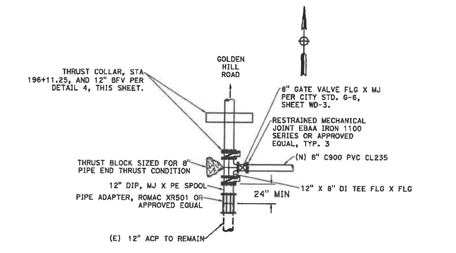
2 WATERLINE TIE-IN DETAIL - GOLDEN HILL ROAD AT ARDMORE ROAD Scale: 1" = 5'
