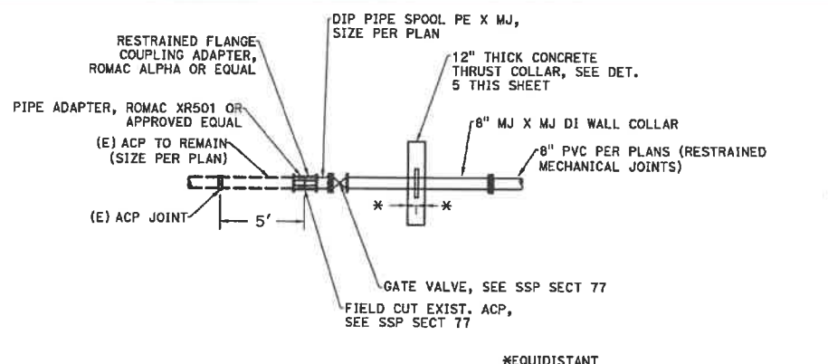
6 VALVE TIE-IN FOR 8" PIPE Scale: NTS
